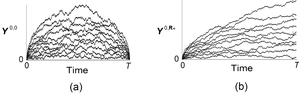
Figure 2. Samples of paths for (a) \mathbf{Y}^{\mathbf{0},\mathbf{0}}(t) and (b) \mathbf{Y}^{\mathbf{0},\mathbb{R}_+}(t) , t \in [0, T] .
