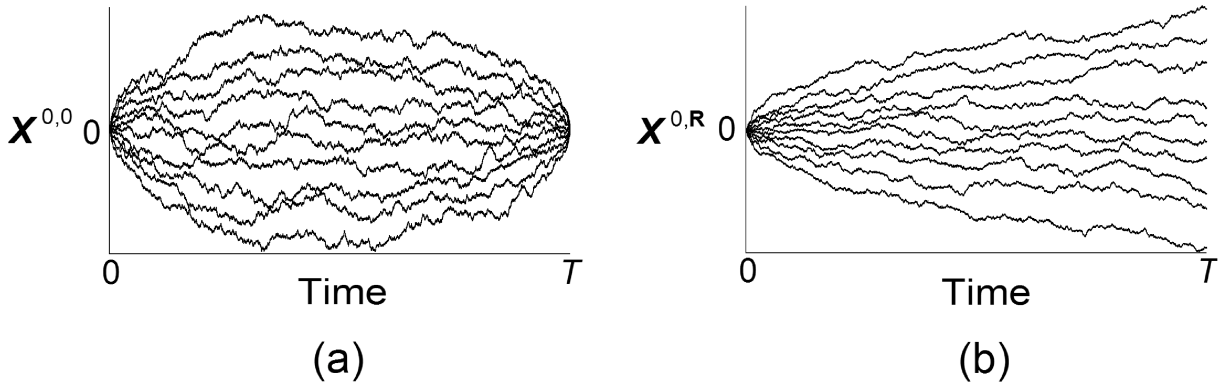
Figure 1. Samples of paths for (a) \mathbf{X}^{\mathbf{0},\mathbf{0}}(t) and (b) \mathbf{X}^{\mathbf{0},\mathbb{R}}(t), t \in [0, T] , generated by simulating the corresponding eigenvalue processes of random-matrix models.
