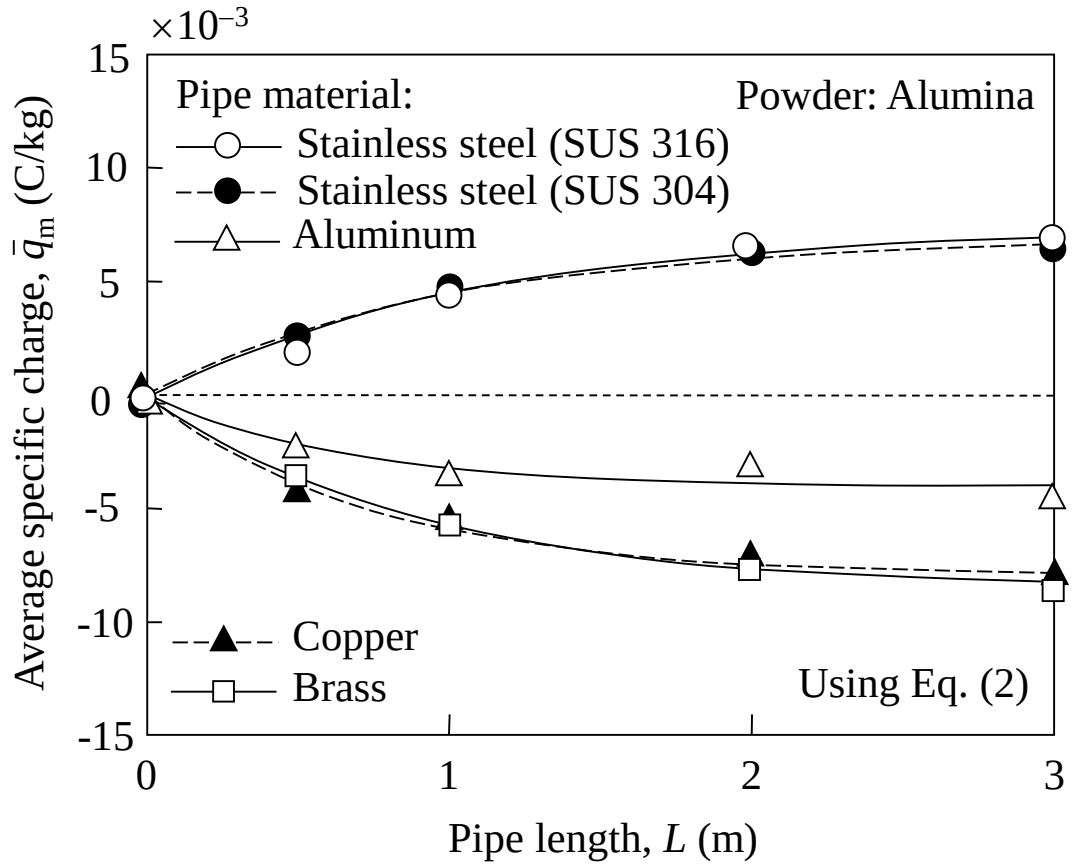
Figure 3. Relationships between average specific charge and pipe length [symbols are experimental data, curves are calculations using (2) and the fitting parameters are listed in Table 1].
