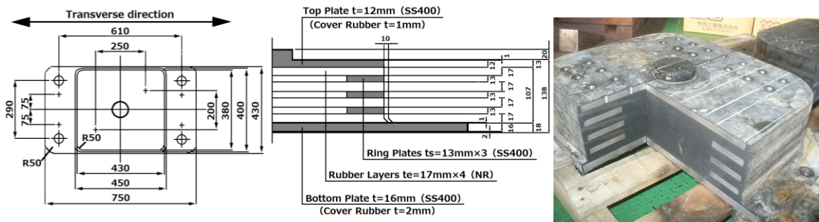
Figure 2.1 Dimensions of ring bearing samples
