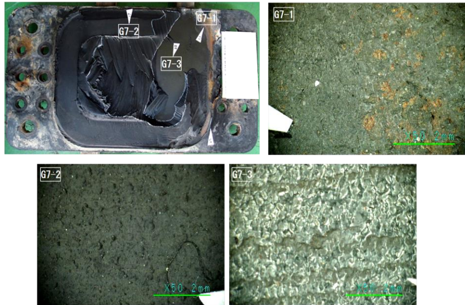
Figure 3.4 Fracture surface of G7
