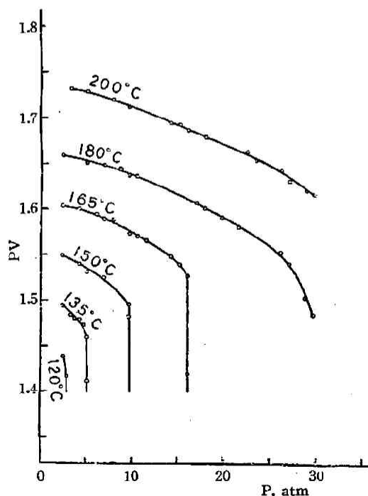
Fig. 4 PV - P curves of mixture. ( \text{C}_2\text{H}_2:\text{CH}_2\text{O} = 1:2 )
