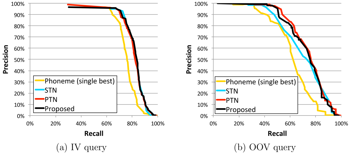
Figure 6.9: Recall-Precision curve.
