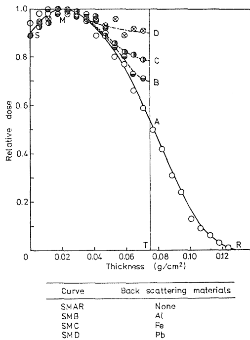
Fig. 5. Relative dose distribution within handsheets for single side irradiation with 0.5 MeV electron beam.
