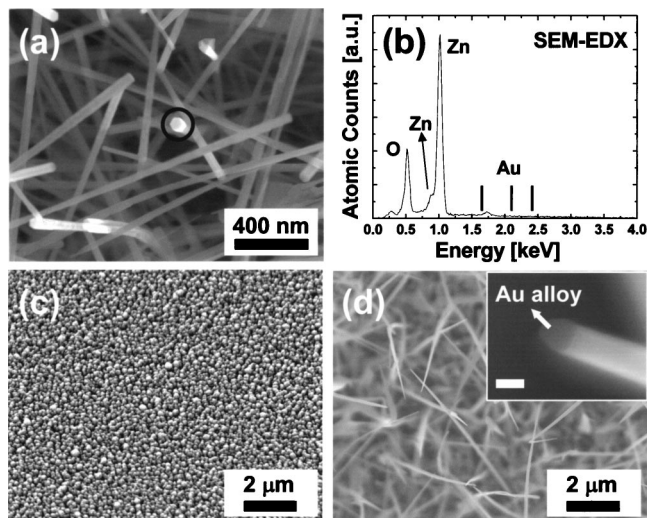
FIG. 2. (a) High-resolution plan-view FE-SEM image of ZnO nanowires grown at 550 °C; (b) SEM-EDX spectrum recorded from the top surface [the point marked by a circle in (a)] of a single nanowire; (c) and (d) show ZnO nanorods (FE-SEM image taken at a tilt angle of 45°) and nanowires (plan-view FE-SEM image) grown on the substrate represented at Fig. 1(a) at 400 and 900 °C, respectively; (d) is a FE-SEM image of a tip area in one of the nanowires grown at 900 °C. Scale bar in the inset indicates 50 nm.
