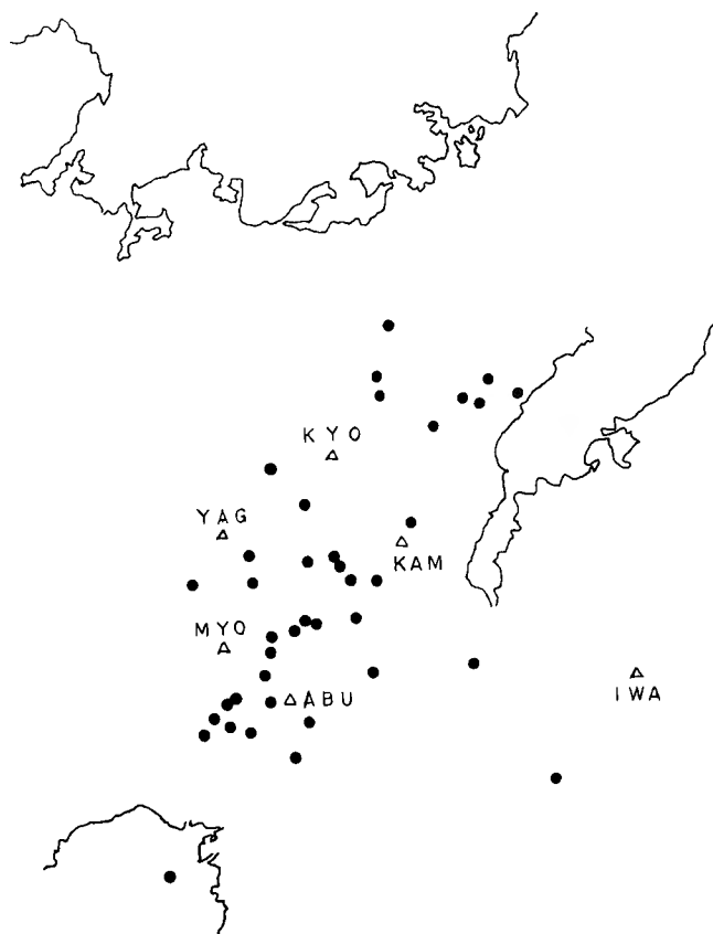
Fig. 6. Distribution of the epicenters of micro-earthquakes. ( V=5.5 km/sec)
