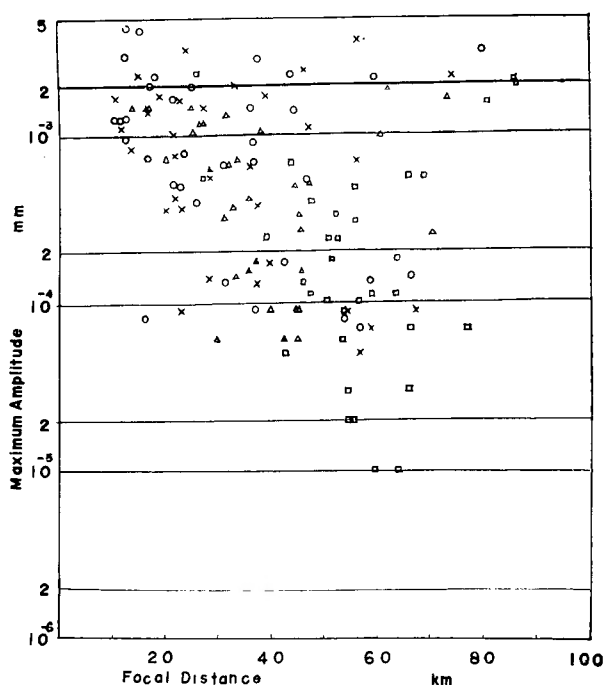
Fig. 10. Relationship between the maximum amplitudes and the hypocentral distances.
