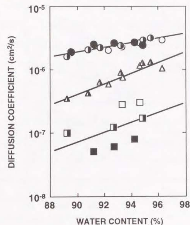
Figure 6.8. Dependence of the diffusion coefficient of (O, ●, ●) glucose, ( \Delta , \Delta ) insulin, and ( \square , \square , \blacksquare ) albumin on the water content in PVA hydrogels with a molecular weight of 2.47 \times 10^5 crosslinked by GA. Open symbols show initial concentration of 2 wt%, half closed symbols of 3 wt%, and closed symbols of 4 wt%.
