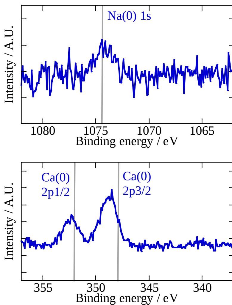
Fig. エラー! メイン文書しかありません。 Results of analysis by XPS for deposits formed on a molybdenum plate after potentiostatic electrolysis at -2.3 V vs. \text{Ag}^+/\text{Ag} in the \text{LiCl-NaCl-CaCl}_2 eutectic melt at 773 K.
