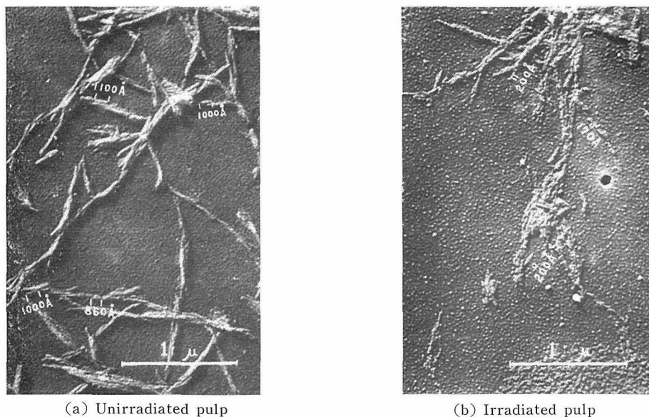
Fig. 2. Electron photomicrographs of residues of hydrolysis at leveling-off point. Many small separated particles which are seen in the photomicrograph (b) of the irradiated pulp would also be the degraded crystallites.
