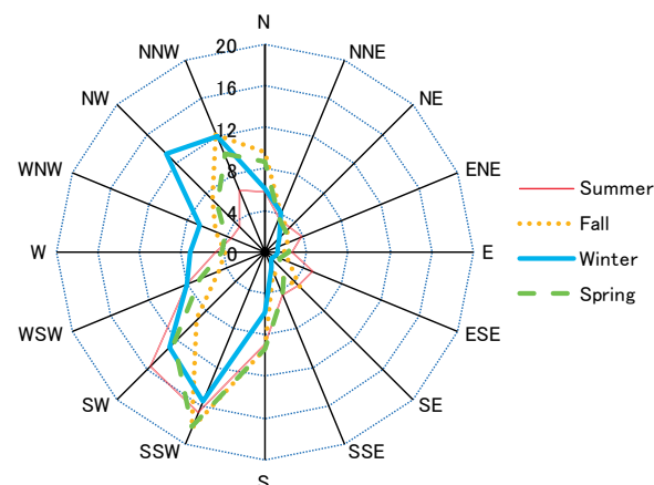
Fig.4 Wind rose in four seasons
