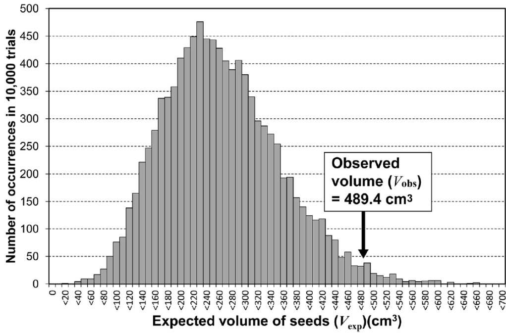
Fig. 2 Distribution of the expected volume of seeds ( V_{exp} ) calculated from 6.7 randomly selected fecal clumps. V_{obs} Total volume of seeds observed in the corpse
