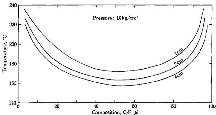
Fig. 5 Effect of vessel diameter on explosion limits at the pressure of 10 kg/cm 2 in C 2 F 4 -O 2 mixtures
