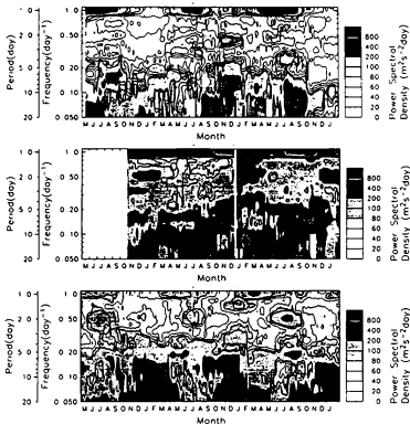
Figure 5.2: Dynamic power spectra of zonal wind velocity in Shigaraki (top), Adelaide (middle) and Saskatoon (bottom) from May 1983 to February 1986. Spectra were analyzed by Fourier transforming an auto-correlation function on a 90 day data series, with a maximum lag of 30 days, where the data window was sled every 5 days.
