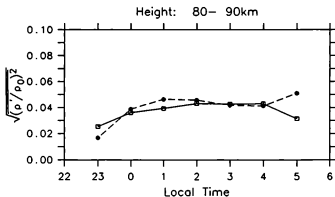
Figure 4.20: Variance of the atmospheric density perturbations calculated for the MU radar (solid line with open squares) and the lidar observations (dashed line with solid circles) [Namboothiri et al. , 1994].
