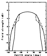
Figure B.1: Computed radiation pattern of the optimized 3-element Yagi's in the infinite array for the case where x-aligned elements are excited. Solid and dashed curves, and chain are for the directions of 0^\circ (x-z plane), 45^\circ , and 90^\circ (x-z plane), respectively [Sato, 1981].
