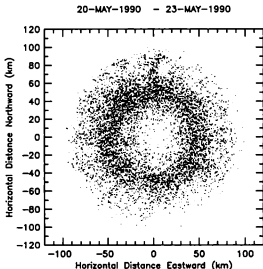
Figure 2.26: An example of horizontal distribution of meteor echoes observed with the MU radar using a doughnut-like transmitting antenna pattern on May 20-23, 1990.
