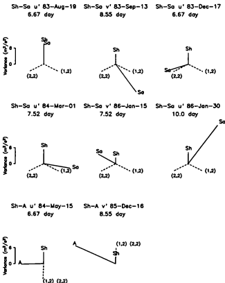
Figure 5.7: Same as Figure 5.5 except for period range of 0.6–10 days. Theoretical phase values are plotted for (1, 2) and (2, 2) modes.
