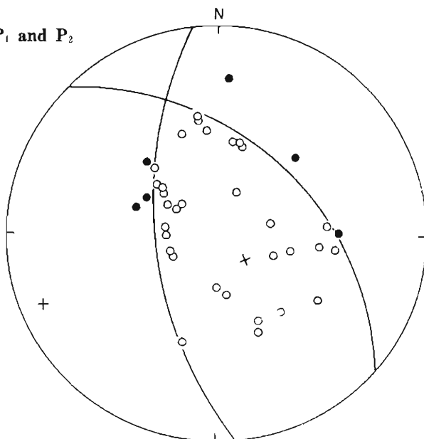
Fig. 5. The radiation pattern of P_1 waves from the first shock. The closed circles, the open circles and the crosses indicate the compressions, dilations and the minimum and maximum principal axes, respectively.
