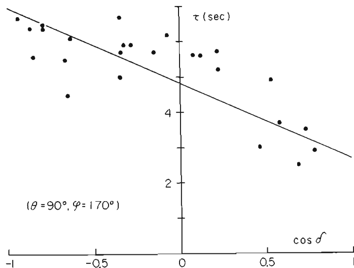
Fig. 7. The relation between the P_1 \sim P_2 interval times and \cos \delta .
