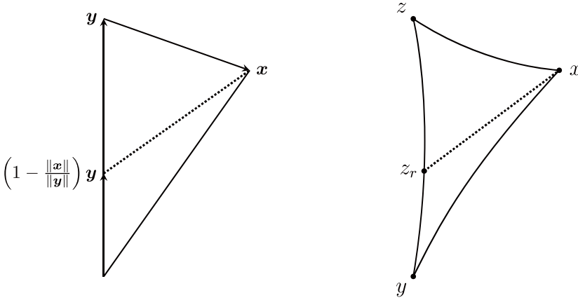
FIGURE 1. A comparison of (3.3) and (3.5)
