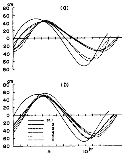
Fig. 10 Tidal curve for present state (a) and dredged state (b).
