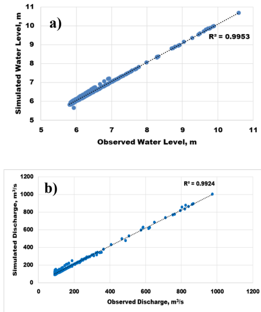
Fig.5: Calibration of a) water-level and b) discharge
