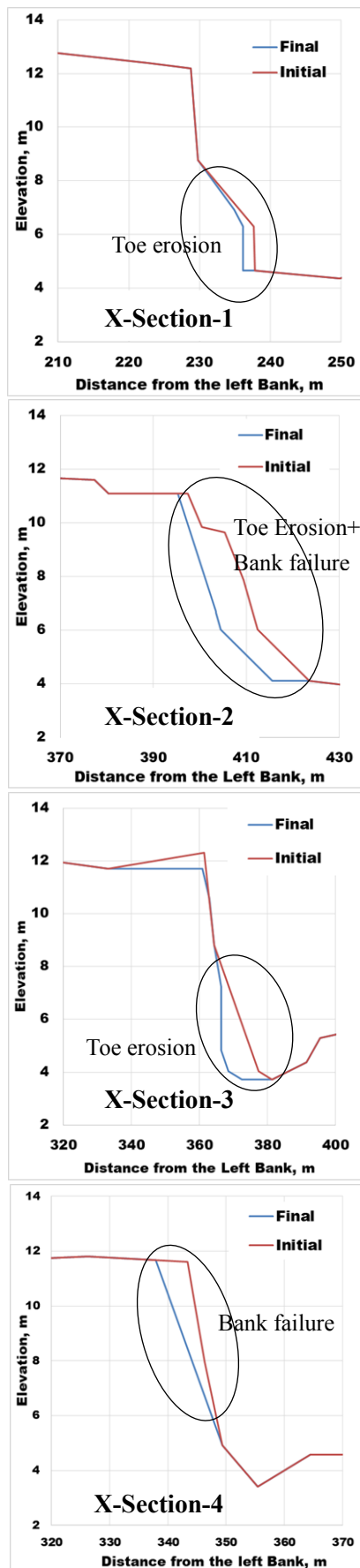
Fig.13 (a-d): Comparison of bank evolution at selected cross-sections
