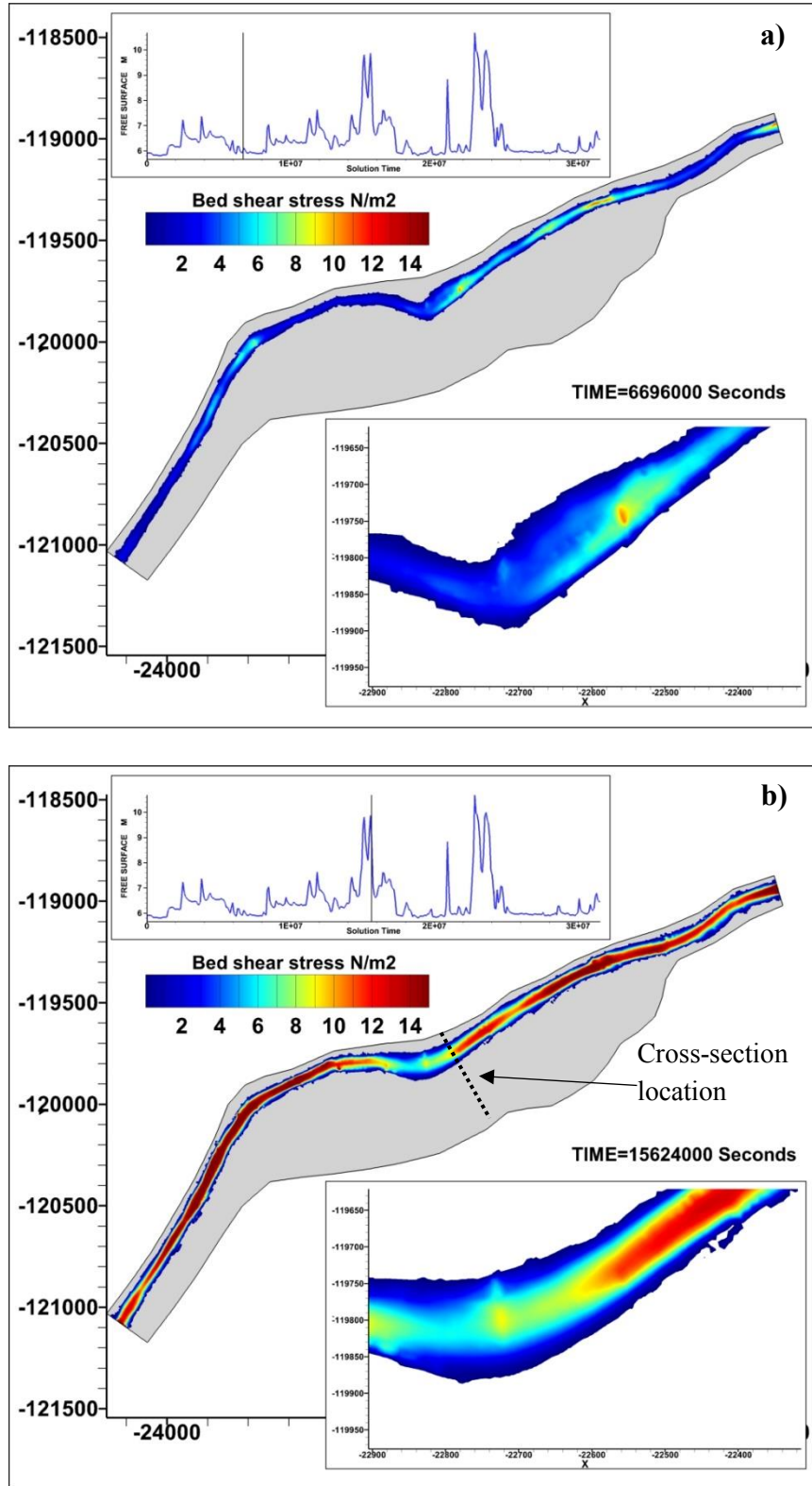
Fig. 8: Bed shear stress ( \tau ) distribution for a) low flow b) high-flow condition
