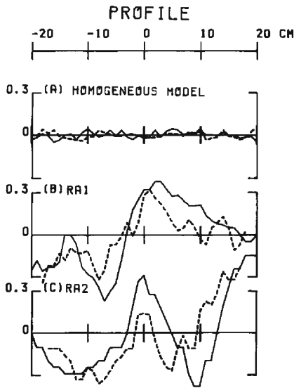
Fig. 7. Phase fluctuation \delta\varphi and amplitude one \delta \ln A_1 along a profile with distance L=70 cm from the source. Solid and dotted lines denote phase and amplitude fluctuations, respectively.
