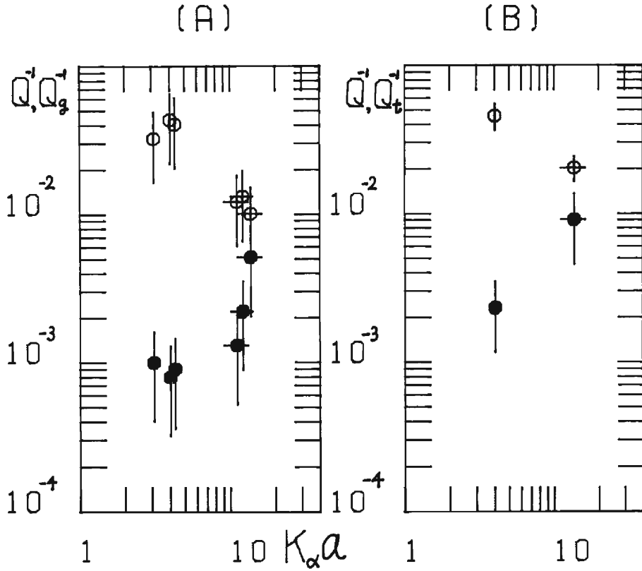
Fig. 9. (A): Dependences of Q_g^{-1} and Q_g^{-1} on k_a a in the preliminary experiment. Open circles and solid ones denote Q_g^{-1} and Q_g^{-1} , respectively. (B): Dependences of Q_i^{-1} and Q_i^{-1} on k_a a in this experiment. Open circles and solid ones denote Q_i^{-1} and Q_i^{-1} , respectively.
