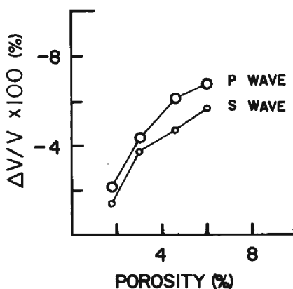
Fig. 3. Relation between rate of decrease of wave velocity, \Delta V/V , and porosity.
