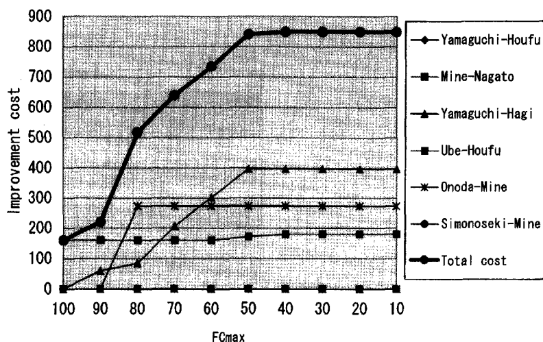
Fig. 8 Relation between FCmax and improvement cost (rock-collapse)
