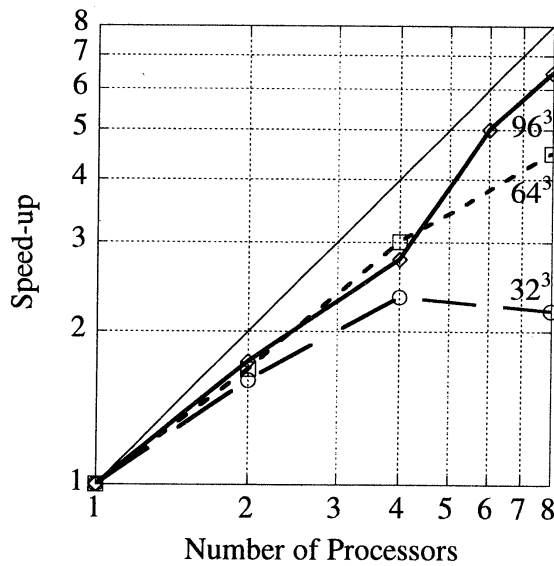
Fig. 4 Parallel performance of FFT PCG method
