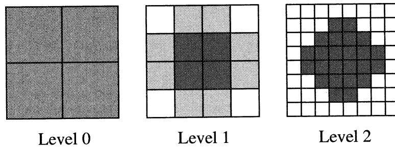
Fig. 2 Multigrid for image-based finite element method
