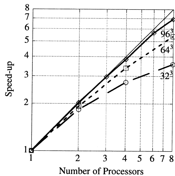
Fig. 5 Parallel performance of CCG method
