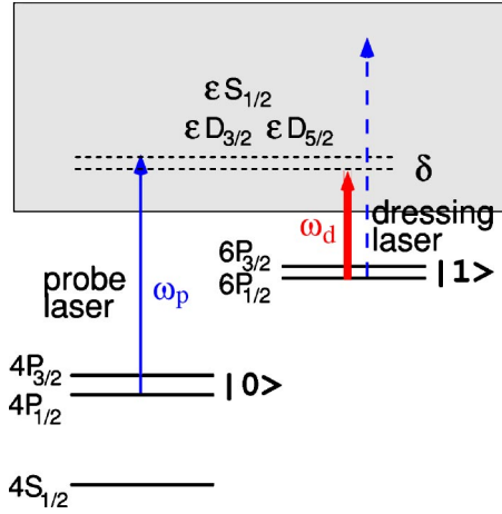
FIG. 1. Level scheme. 4p and 6p states of K atom are coupled by the linearly polarized probe and dressing lasers. With the laser intensities and the detuning range we have chosen for the present study, it is possible to consider each set of the fine-structure-resolved system, the K 4p_{1/2} - 6p_{1/2} system and the K 4p_{3/2} - 6p_{3/2} system. Incoherent ionization from state |1\rangle by the probe laser is also shown by the dashed line.
