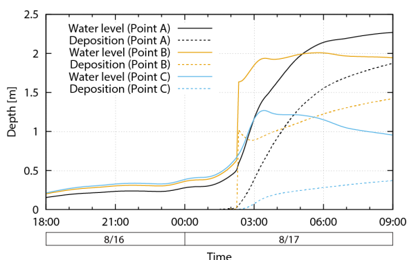
Fig.9 Water level and deposition depth at 3 points in Sakiyama river watershed
