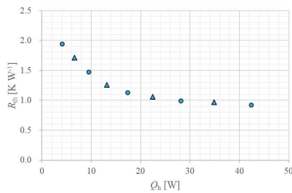
Fig. 1 Variation of thermal resistance with heat input.
