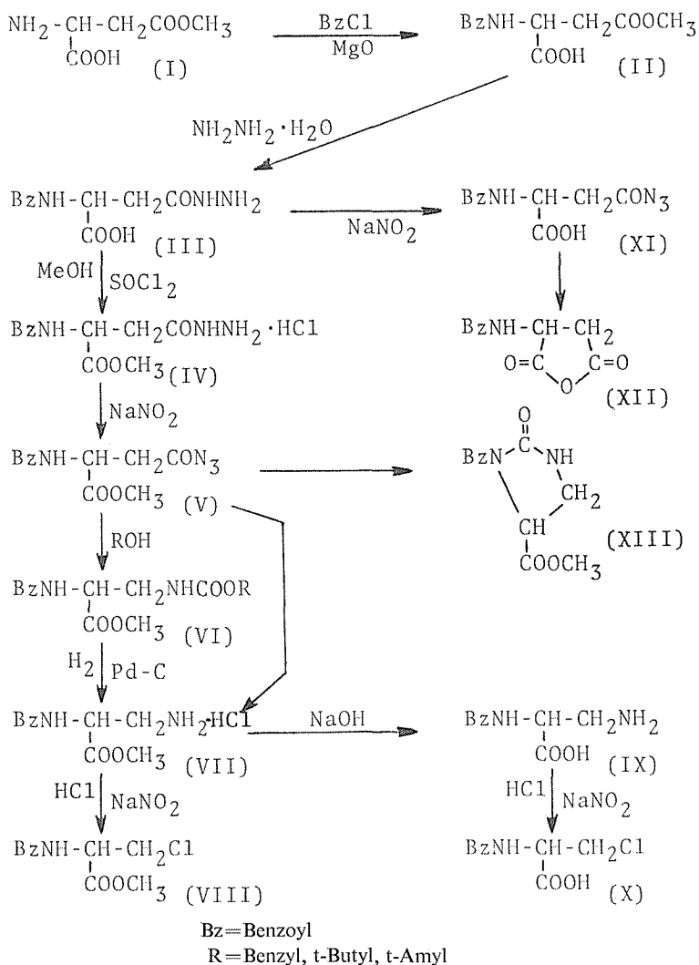
Reaction Scheme
