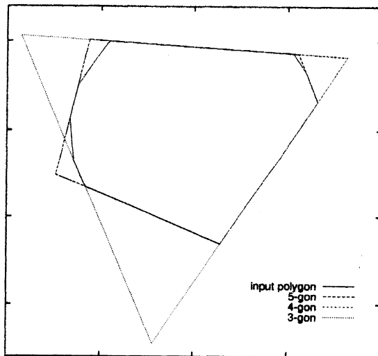
Fig. 2 Result of optimal algorithm
