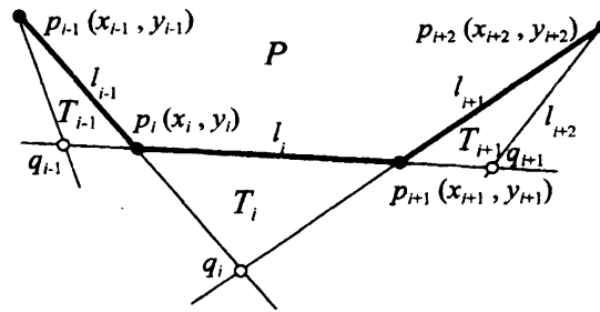
Fig. 1 cross point q_i and added triangle T_i
