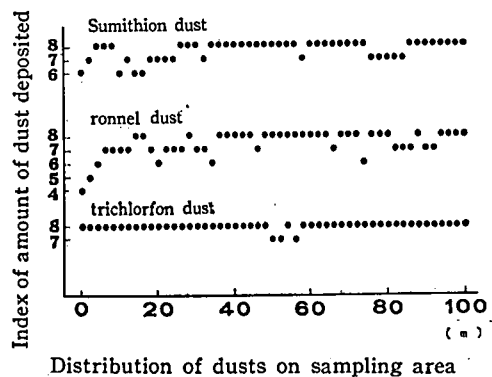
Fig. 2. Distribution of dusts deposited by helicopter aerial dusting. (emission rate is 6 kg/10a.)
