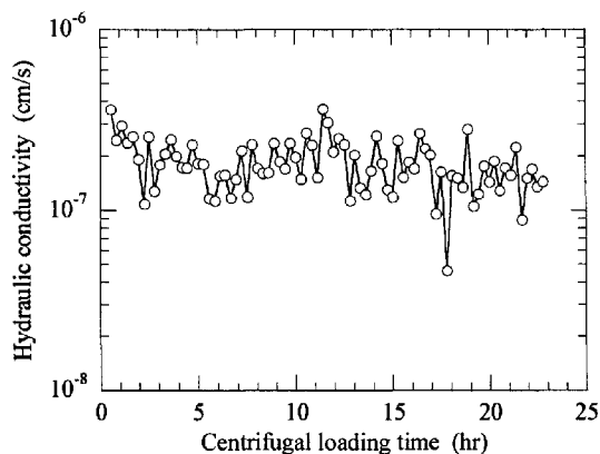
Fig. 15 Change of hydraulic conductivity for the centrifugal loading time (case of PS)
