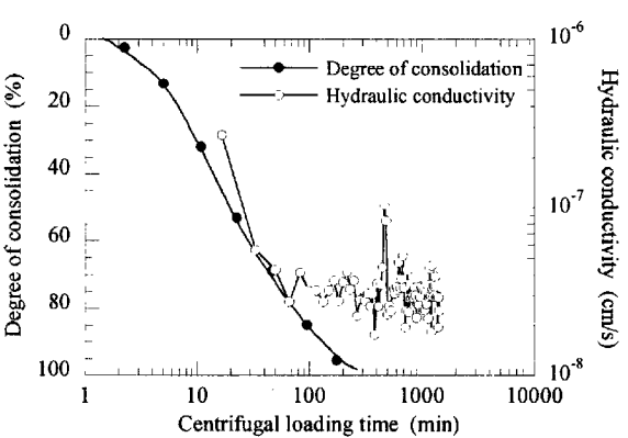
Fig. 21 Change tendency of consolidation and hydraulic conductivity (case of CS)
