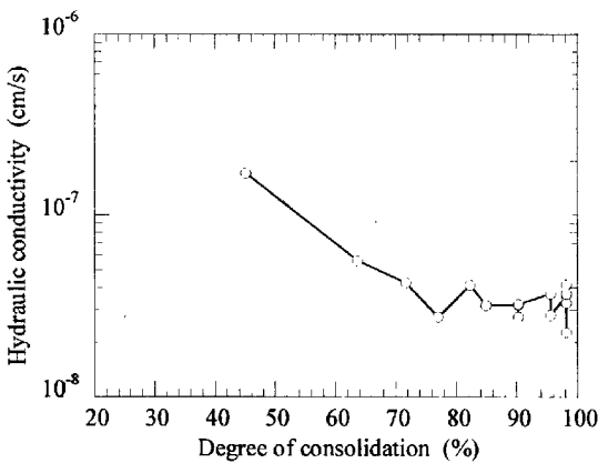
Fig. 22 Relationship between hydraulic conductivity and degree of consolidation (case of CS)
