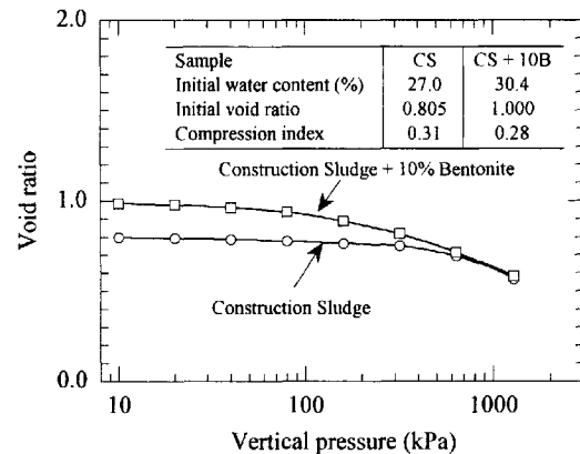
Fig. 8 e-log p curves of CS
