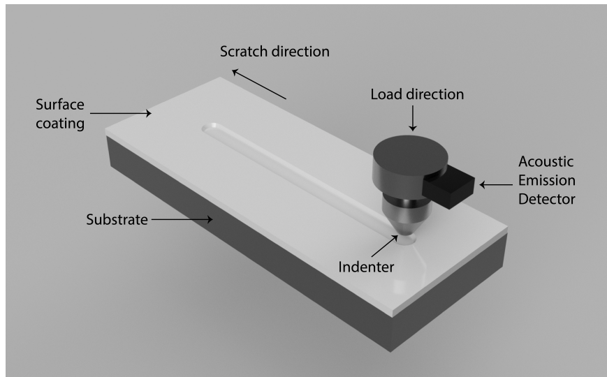
Figure 2. Simplified schematic of the Revetest Scratch Tester (RST).
