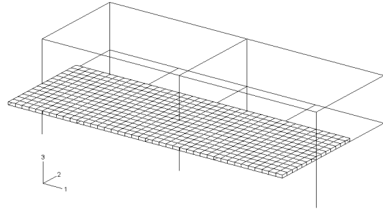
Fig. 12 FE model of test structure
