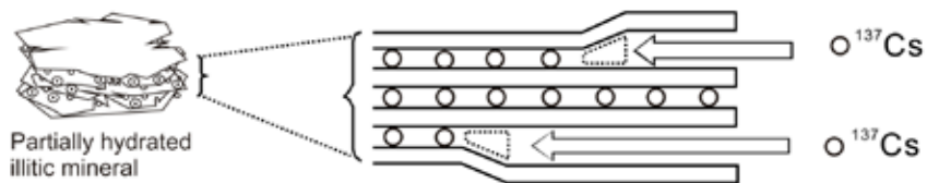
Figure 5. Schematic diagrams of illitic minerals intercalated by hydroxy-Al polymers in their expanded interlayer sites at pH 4.0-5.0, followed by the decreasing accessibility of ^{137}\text{Cs} to the frayed-edge site (a). At strongly acidic soil condition, the hydroxy-Al polymers can be monomerized, enabling ^{137}\text{Cs} to access the frayed-edge site (b)
