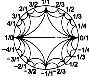
Figure 2: Farey tessellation
