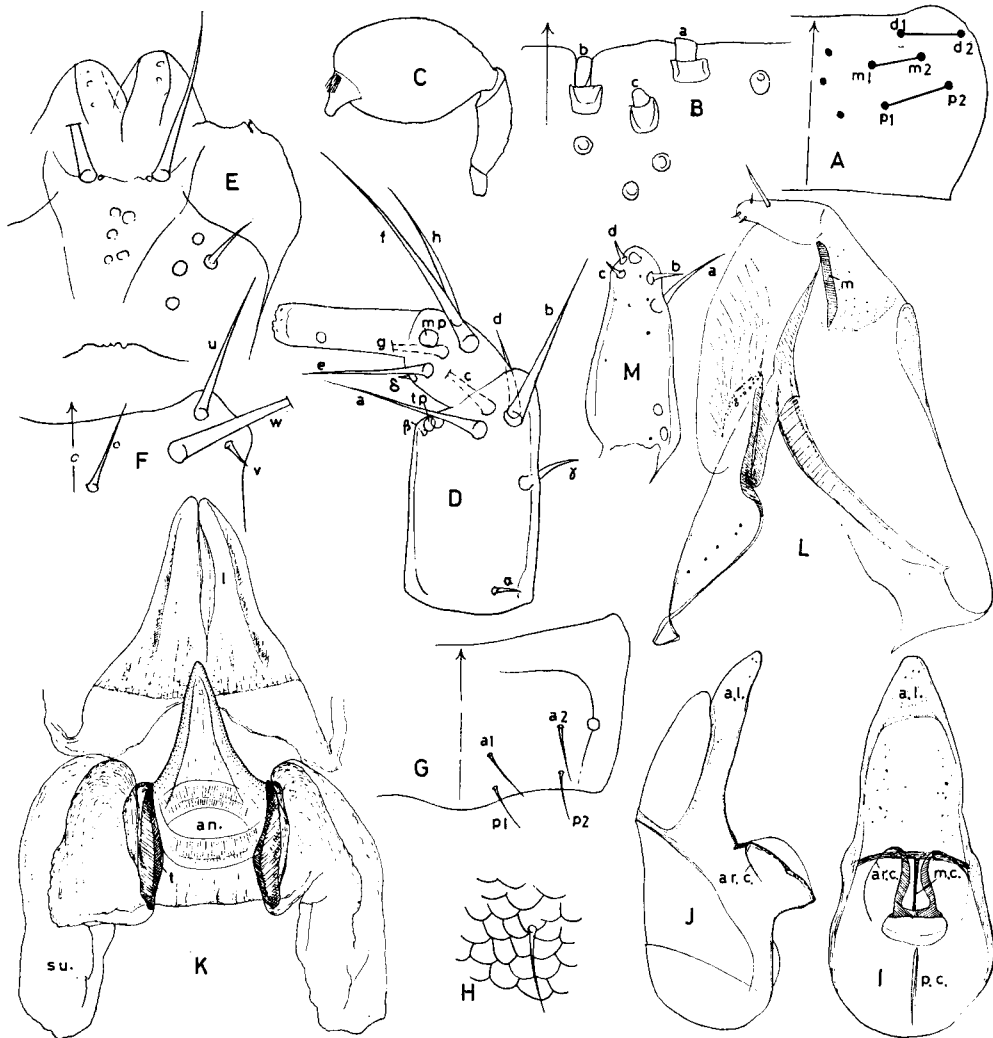
Fig. 46. Callicerus obscurus GRAV. from Leipzig. A, Labral chaetotaxy; B, Labral margin; C, Maxillary palpus; D, Labial palpus; E, Glossa & prementum; F, Mentum; G, H, \delta terg. VIII & its microsculpture; I, J, Median lobe; K, Inner armature of aedeagus; L, M, Lateral lobe.
