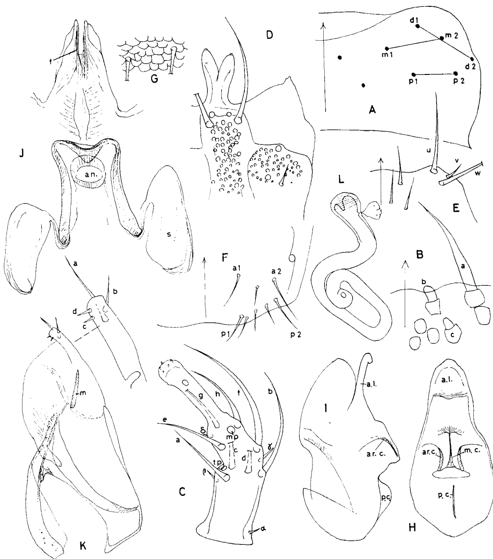
Fig. 35. Atheta ( Psammotiba ) kamtschatica BRUNDIN from Miyako, Pref. Iwate. A, Labral chaetotaxy; B, Labral margin; C, Labial palpus; D, Glossa & prementum; E, Mentum; F, G, ♂ terg. VIII & its microsculpture; H, I, Median lobe; J, Inner armature of aedeagus; K, Lateral lobe; L, Spermatheca.
