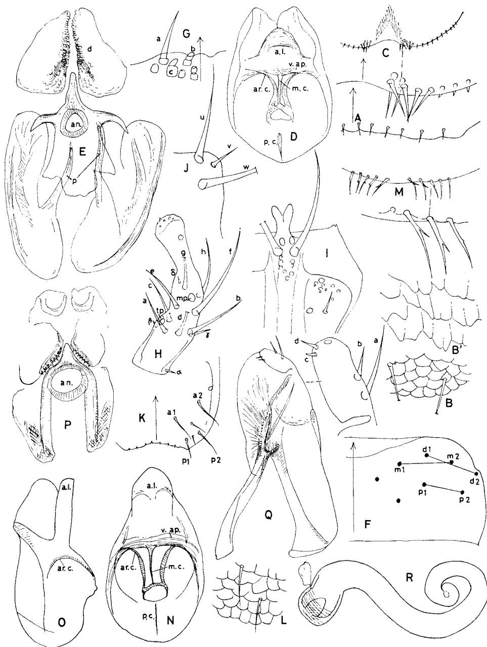
Fig. 36. Atheta (Halostiba) ushio (K. SAWADA) from Wakasa-Takahama, Pref. Fukui. A , Marginal setulae of \delta terg. VIII; B , B' , Microsculpture of \delta terg. VIII & its underside ( B' ) reticulation; C , \delta stern. VIII; D , Median lobe; E , Inner armature of aedeagus. Atheta (Halostiba) magnipennis BERNHAUER from Wakasa-Takahama, Pref. Fukui. F , Labral chaetotaxy; G , Labral margin; H , Labial palpus; I , Glossa & prementum; J , Mentum; K , L , \delta terg. VIII & its microsculpture; M , Marginal setae of \delta stern. VIII; N , O , Median lobe; P , Inner armature of aedeagus; Q , Lateral lobe; R , Spermatheca.
