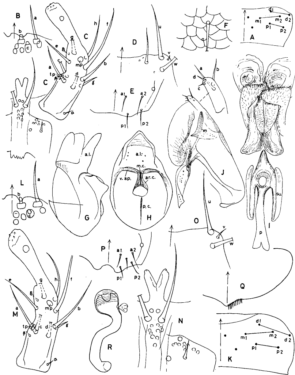
Fig. 32. Atheta ( Anopleta ?) ravilla (ERICHSON) from Austria. A, Labral chaetotaxy; B, Labral margin; C, Labium; D, Mentum; E, F, ♂ terg. VIII & its microsculpture; G, H, Median lobe; I, Inner armature of aedeagus; J, Lateral lobe.
