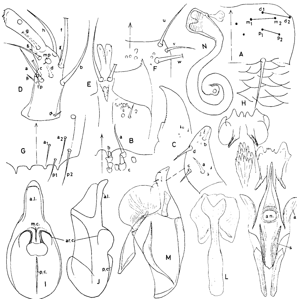
Fig. 5. Atheta (Xenota) grata CAMERON from Kurume. A, Labral chaetotaxy; B, Labral margin; C, Right mandible; D, Labial palpus; E, Glossa & prementum; F, Antenna; G, H, 8th sternite & its microsculpture; I, J, Median lobe; K, Inner armature of aedeagus; L, Ventral plate of copulatory piece; M, Lateral lobe; N, Spermatheca.
