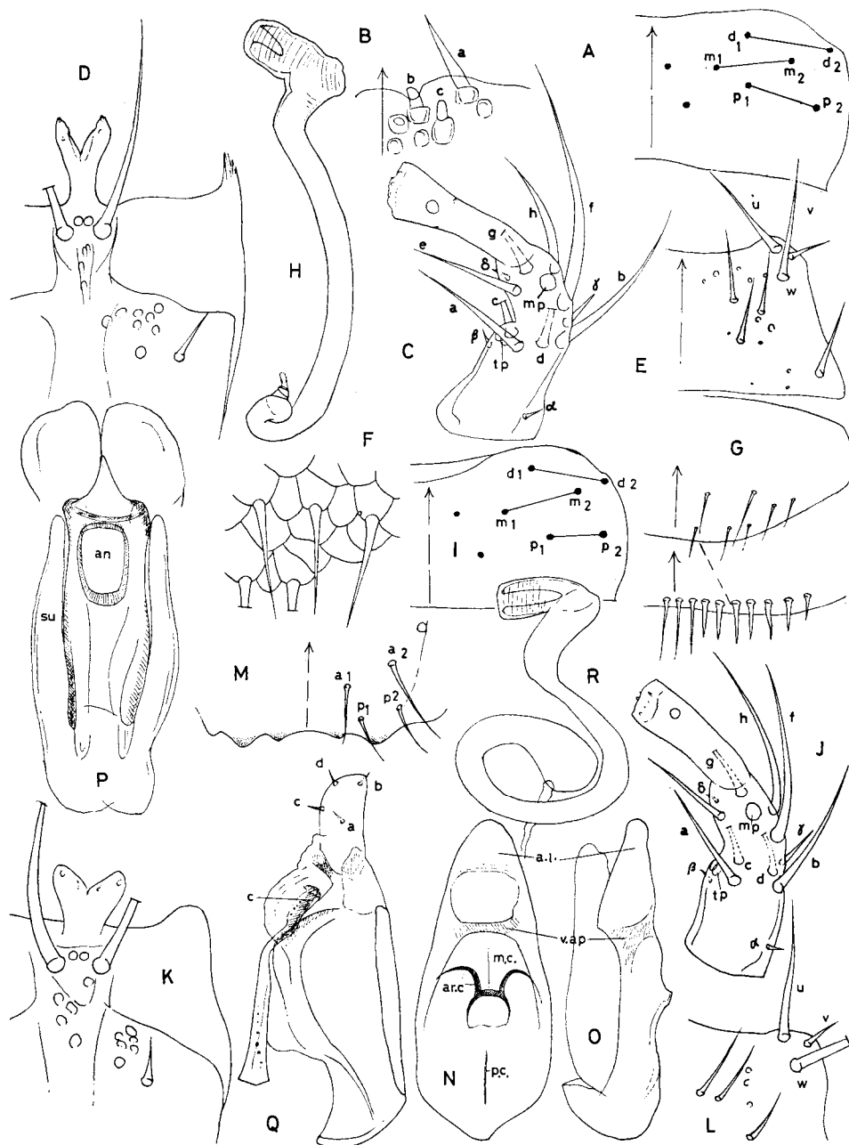
Fig. 2. Atheta ( Datomicra ) celata (ERICHSON) from Hamburg. A, Labral chaetotaxy; B, Labral margin; C, Labial palpus; D, Glossa & prementum; E, Mentum; F, Microsculpture of terg. VIII; G, ♀ stern. VIII; H, Spermatheca.
