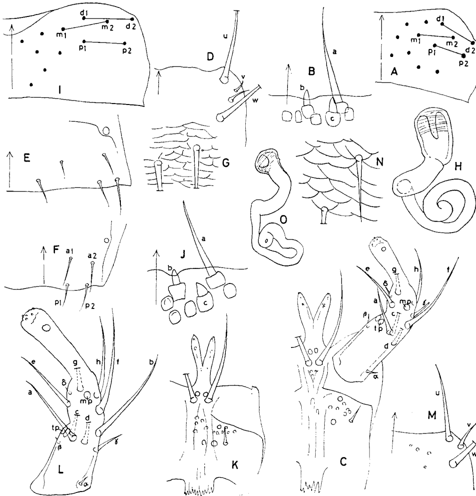
Fig. 30. Atheta ( Plataraea ) dubiosa BENICK from Germany. A, Labral chaetotaxy; B, Labral margin; C, Labium; D, Mentum; E, Chaetotaxy of terg. III; F, G, ♀ terg. VIII & its microsculpture; H, Spermatheca. Atheta ( Plataraea ) nigritula (GRAVENHORST) from Germany. I, Labral chaetotaxy; J, Labral margin; K, Glossa & prementum; L, Labial palpus; M, Mentum; N, Microsculpture of terg. VIII; O, Spermatheca.
