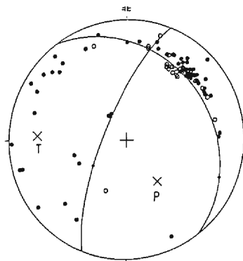
Fig. 5. Focal mechanism of the earthquake on March 18, 1987 by the JMA. (lower hemisphere of equal area projection)
