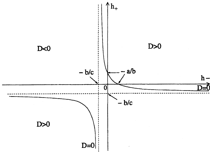
Figure 3: \kappa_* l > \pi/2, a > 0, b < 0, c < 0
