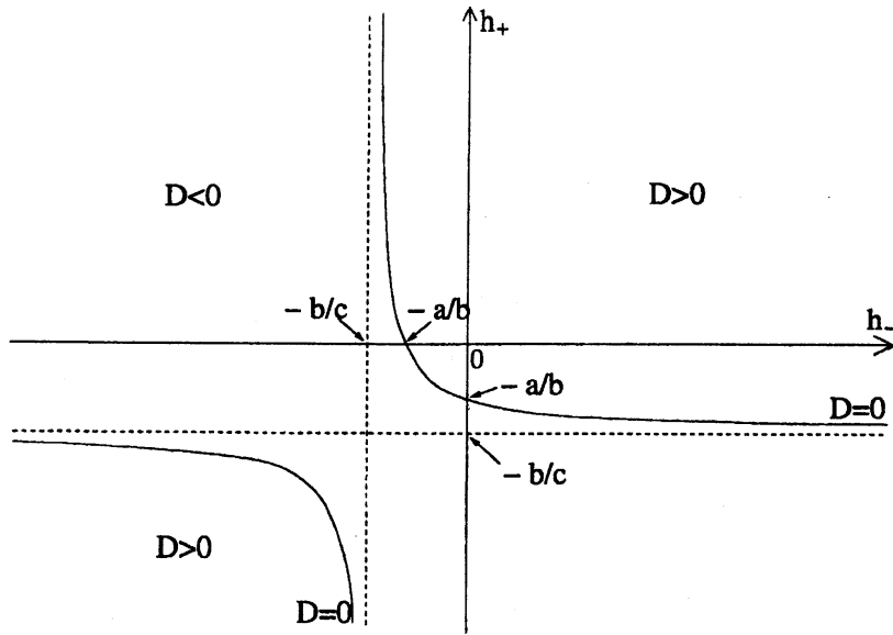
Figure 1: \kappa_* l < \pi/2, a < 0, b < 0, c < 0
