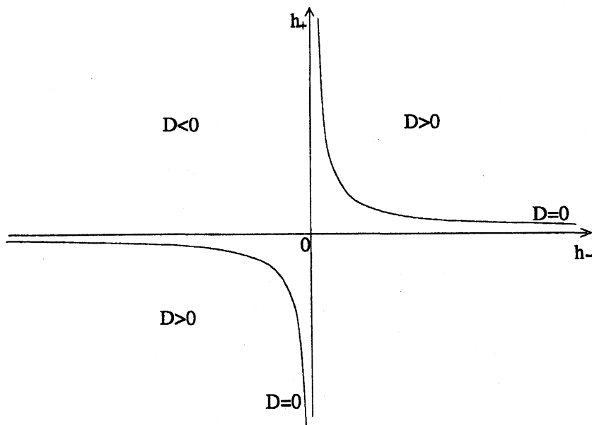
Figure 4: \kappa_* l > \pi/2, a > 0, b = 0, c < 0
