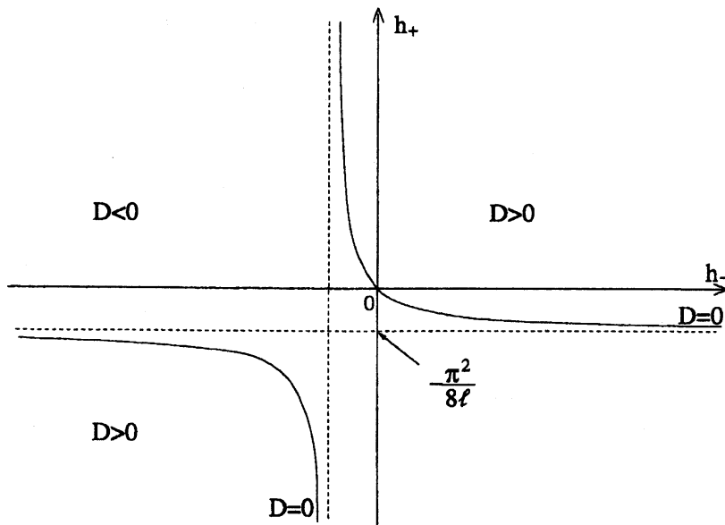
Figure 2: \kappa_* l = \pi/2, a = 0, b = -\kappa_* l, c = -2/\kappa_*
