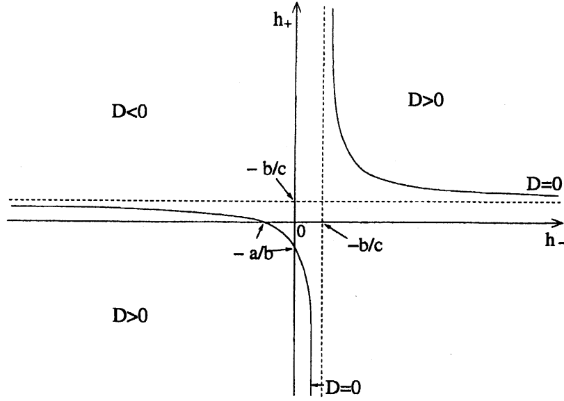
Figure 5: \kappa_* l > \pi/2, a > 0, b > 0, c < 0
