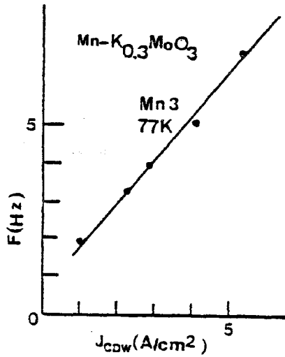
Fig.9 : Voltage oscillations frequency as a function of excess CDW current density in a Mn-doped sample at 77 K.
