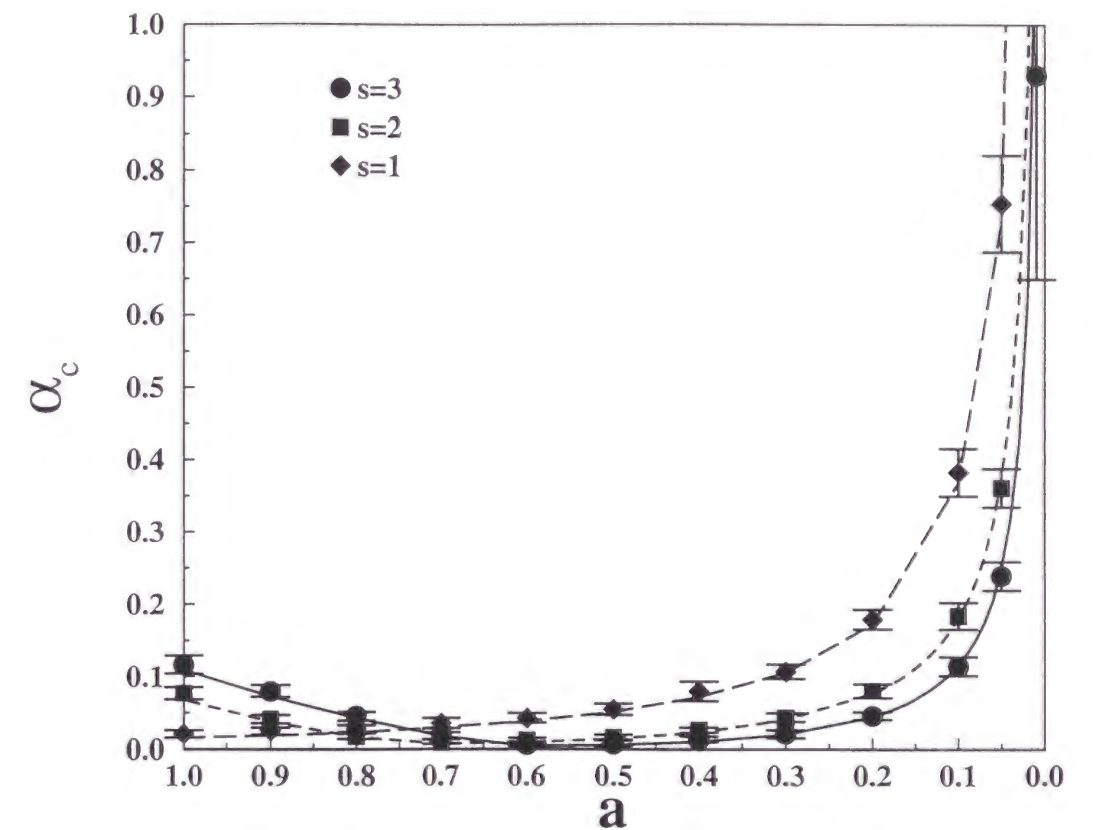
Figure 3.3: Storage capacity \alpha_c as a function of the mean activity level a for a threshold H = 0.5 and mixed numbers s = 1, 2, 3 . The data points indicate numerical results with N = 2000 for 20 trials. The lines were obtained from theoretical analysis.
