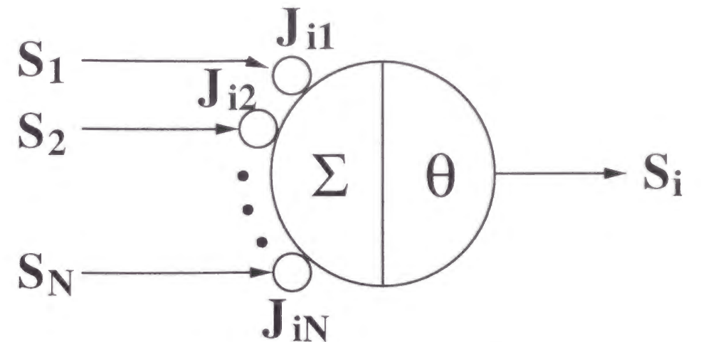
Figure 1.2: McCullo-Pitts neuron
