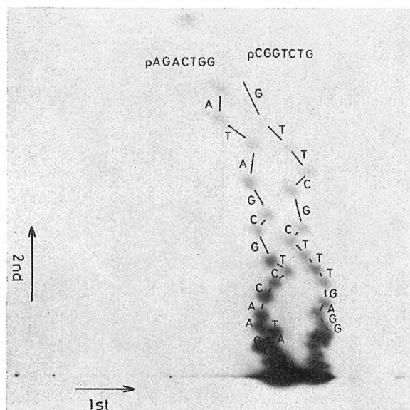
Fig. 6. A fingerprint of partial enzymatic digests derived from HapD-HgaI labelled at both 5'-ends.
