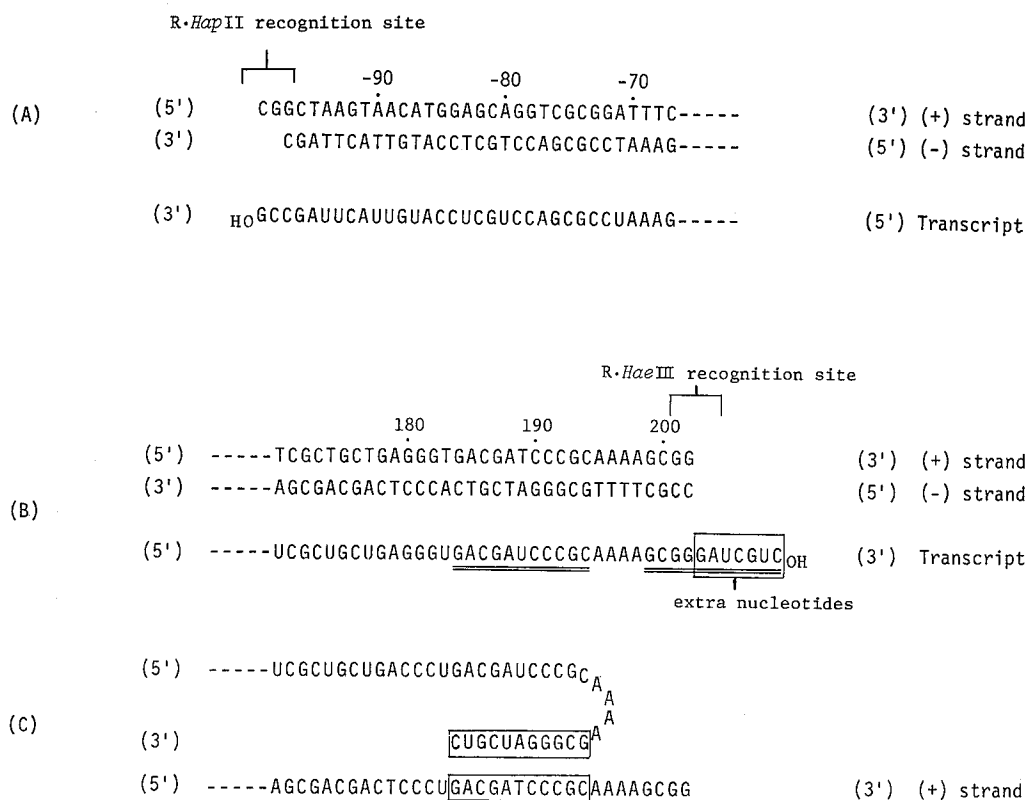
Fig. 4. The sequences deduced for the HapII end (A) and the HaeIII end (B) of HapC-HaeI .
