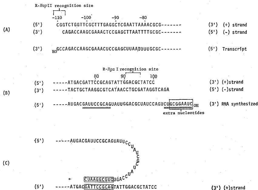
Fig. 7. The sequences deduced for the HapII end (A) and the HgaI end (B) of HapD-HgaI.
