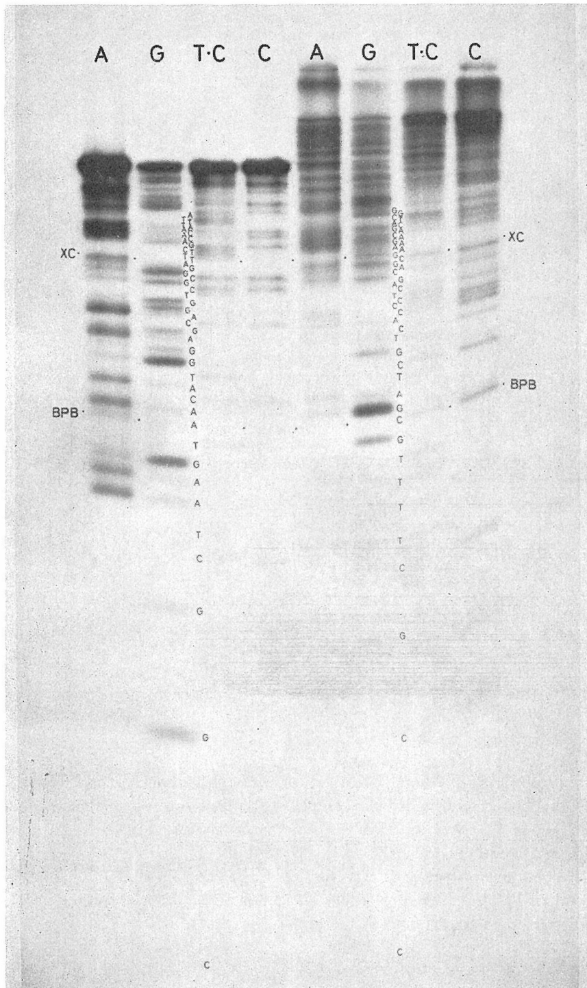
Fig. 2. Autoradiograms of sequencing gels prepared by the method of Maxam and Gilbert. 15)
