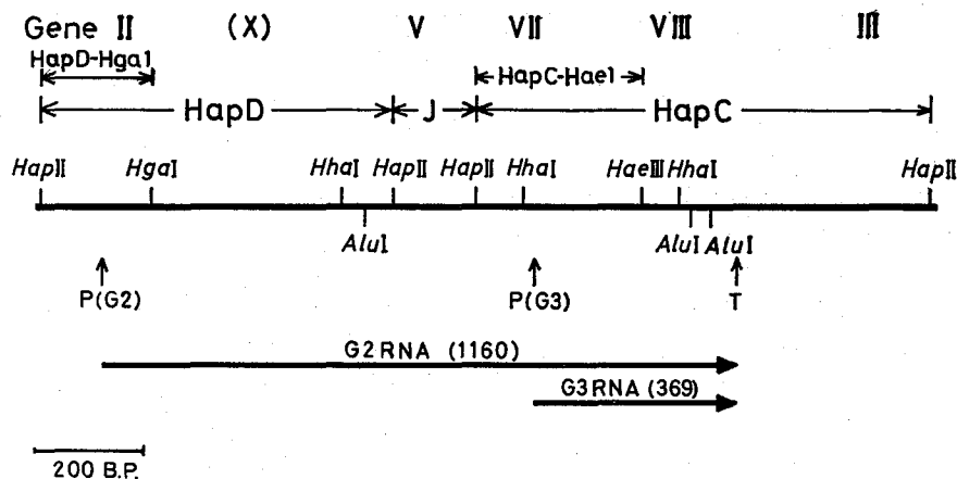
Fig. 1. Cleavage and transcription maps in the HapD to HapC region of bacteriophage fd. Restriction endonucleases HapII , HaeIII , HgaI , and HhaI were prepared from H. aphrophilus , H. aegyptius , H. gallinarum and H. haemolyticus , respectively. Data were taken from ref. 8.
