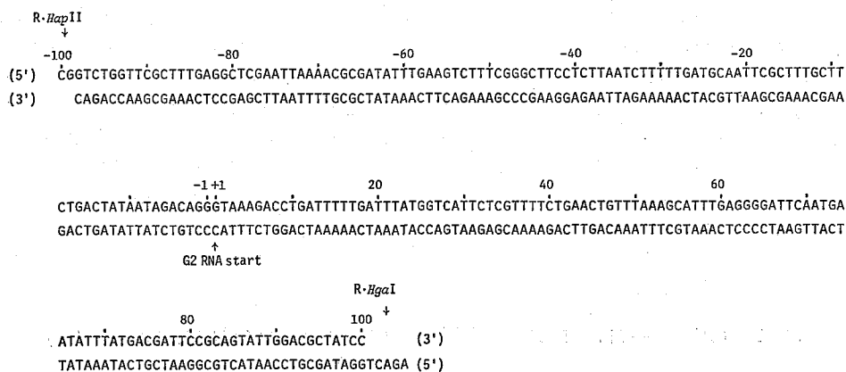
Fig. 8. The total sequence of HapD-HgaI.
