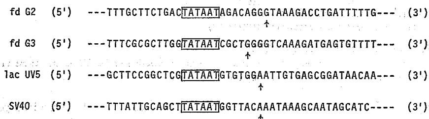
Fig. 9. Comparison of the sequences of four high level promoters with vertically aligned with reference to the TATAAT sequence and with transcription oriented from left to right.
