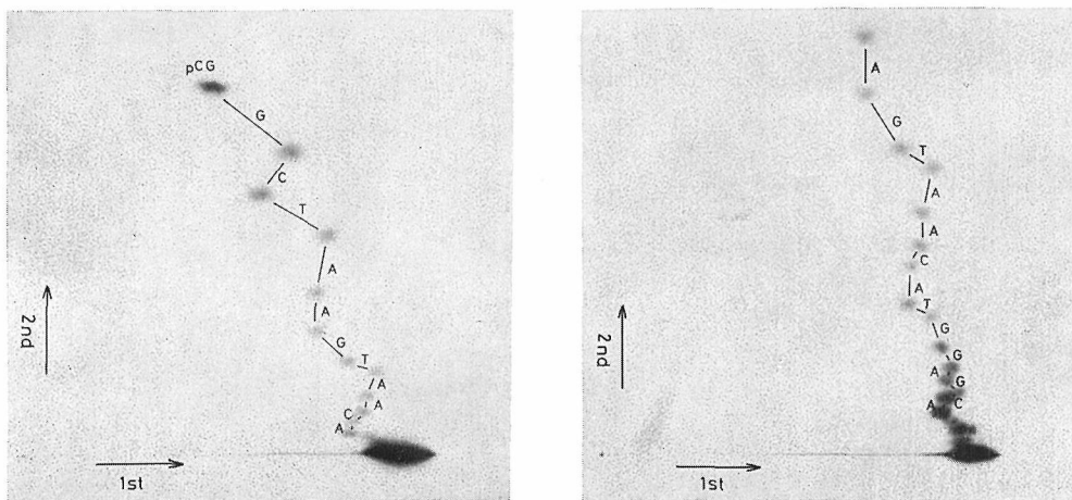
Fig. 3. Fingerprints of partial enzymatic digests derived from the Hap II end of HapC-Hae I.
