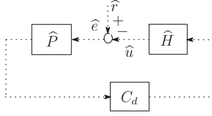
Figure 4.3: Doubly sensitivity-preserving (DSP) discretized system \hat{\Sigma} .
