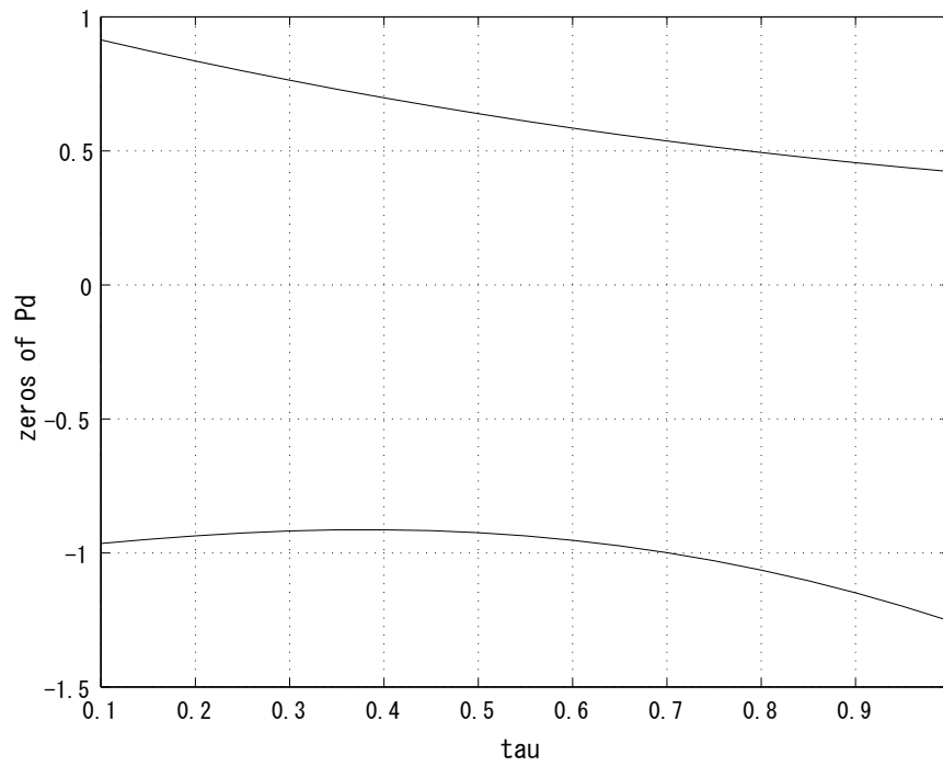
Figure 4.6: Zeros of naively discretized plant P_d(z) .
