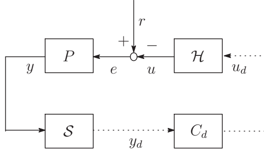
Figure 4.1: Sampled-data system \Sigma .
