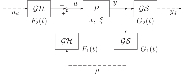
Figure 5.1: Sampled-data system using time-sharing multirate sample-and-hold controllers.
