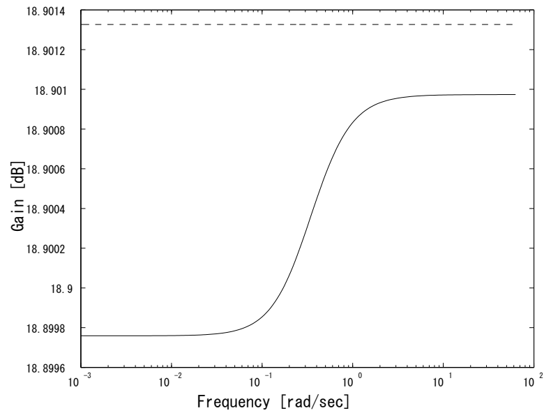
Figure 5.10: Frequency response gain of \underline{Q}(j\varphi) (solid line) and \frac{1}{k^*} (dashed line).
