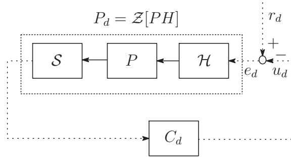
Figure 4.2: Naively discretized system \Sigma_d .
