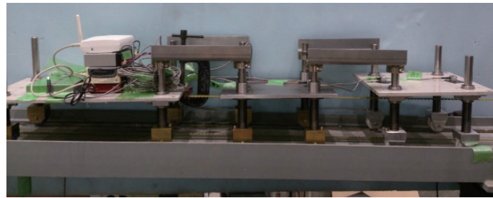
Fig. 2. (Color online) Tractor-trailer system: (a) drawing with sensor layout (marked in blue) (unit: mm) and (b) photo.
