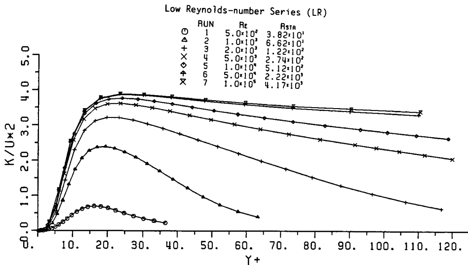
Figure 17. Calculated distribution of turbulent energy in the wall region.
