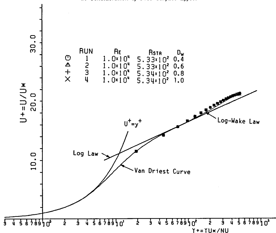
Figure 6. Effect of free-surface damping factor D_w on mean velocity distribution.
