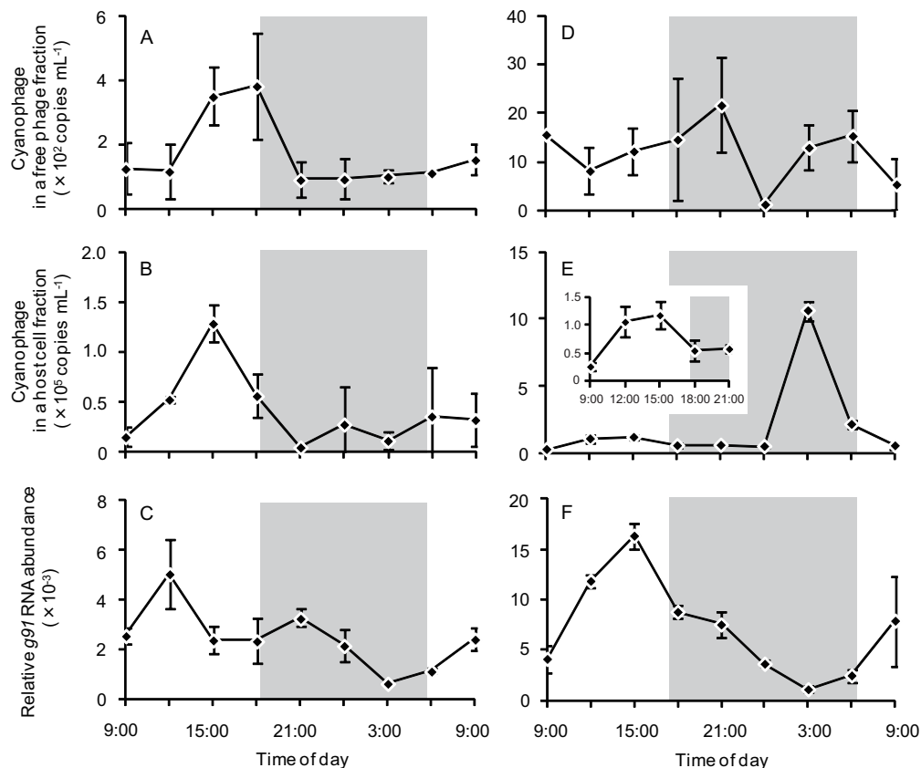
Fig. 3. Diel changes in the abundances of cyanophage in both the free phage (A and D) and the host cell (B and E) fractions determined by g91 real-time PCR in Hiro Sawanoike Pond on 15 Sep (A and B) and 21 Oct (D and E). Diel change of expression of the cyanophage g91 RNA within the infected host cells in Hiro Sawanoike Pond on 15 Sep (C) and 21 Oct (F). g91 relative expression was determined by real-time PCR and by dividing the numbers of RNA copies from the cyanophages by the number of copies in the host M. aeruginosa determined using the mpB primer set. Points represent averages of three experiments and the error bars indicate the standard deviations of three experiments. The grey shaded areas indicate the periods of darkness. The inset in panel E is a magnification of the abundances of cyanophage in the host cell fraction from 09:00 to 21:00 on 21 Oct.
