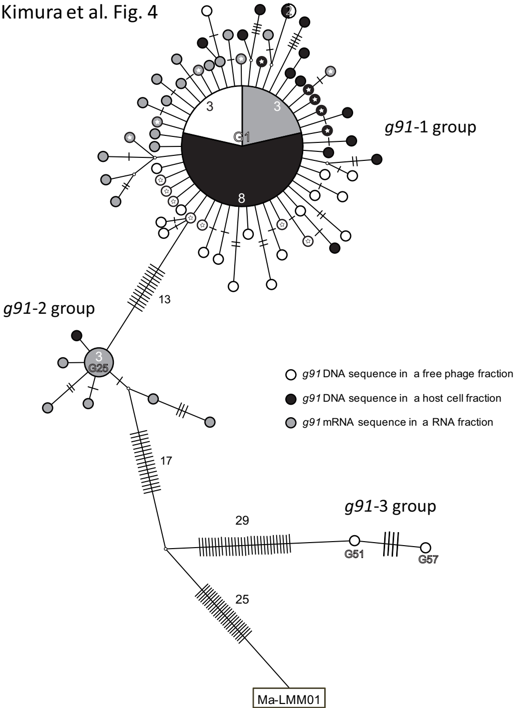
Fig. 4. Maximum parsimony network performed using the TCS v1.21 program (7) for the cyanophage g91 genotypes. The areas of the circles are roughly proportional to the number of times a sequence was found. The number of nucleotide differences between two genotypes is the sum of steps for the shortest connecting path, summing cross-hatches, intervening genotypes, and junction nodes (small circles). A star symbol indicates the genotype had a silent mutation compared to the G1 type sequence.
