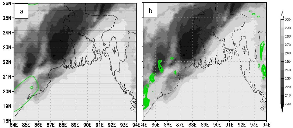
Fig 5. Shaded black body temperature TBB and contoured specific humidity gradient (a) ( \geq 3 \text{ g/kg/100km} ) using JRA-25 data; (b) ( \geq 10 \text{ g/kg/100km} ) by GSM on 12 UTC 4th April, 2011
