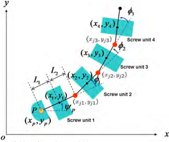
Fig. 9. Definition of coordinate variables
