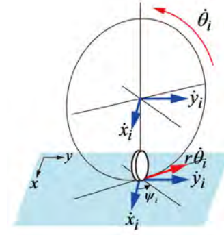
Fig. 10. Velocities generated for a passive wheel
