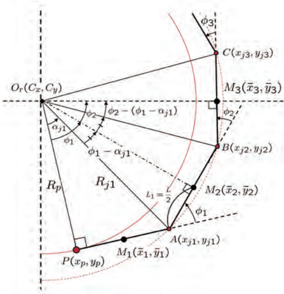
Fig. 19. Configuration asymptotically achieved for constant curvature
