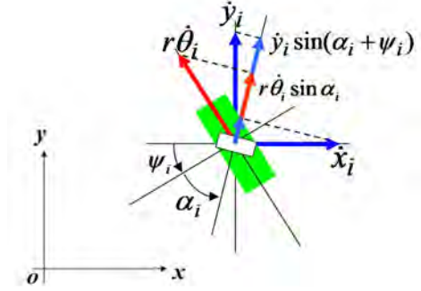
Fig. 11. Velocity constraint for a passive wheel (top view)
