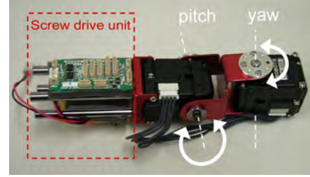
Fig. 3. Joint unit
