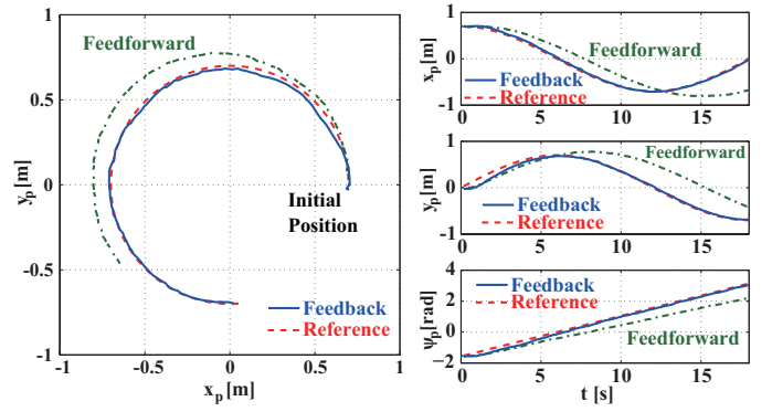
Fig. 14. Experimental results for fixed joint angles (feedback & feedforward)
