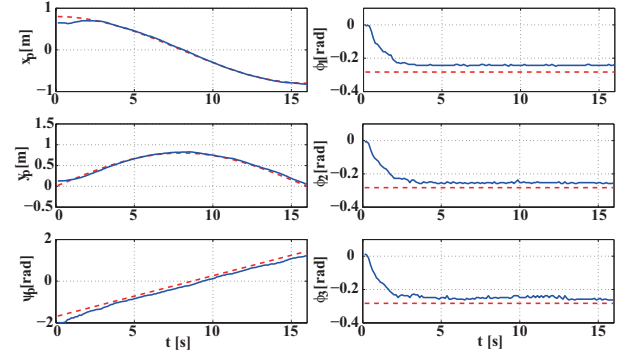
Fig. 16. Time responses of the state variables in experiment (feedback)
