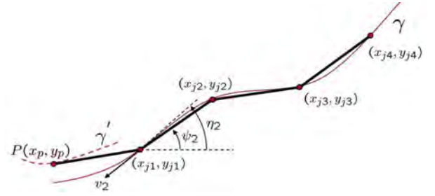
Fig. 17. Target path \gamma and joint positions
