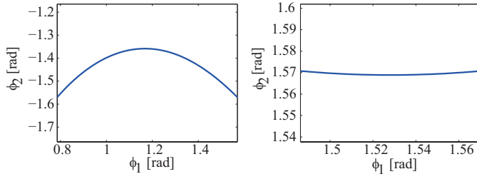
Fig. 25. (\phi_1, \phi_2) for which A does not have full column rank. (Left: \phi_1 > 0 , \phi_2 < 0 , Right: \phi_1 > 0 , \phi_2 > 0 )
