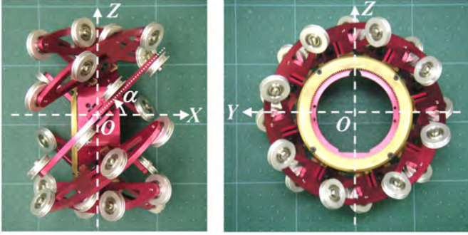
Fig. 6. Side and front views of a screw
