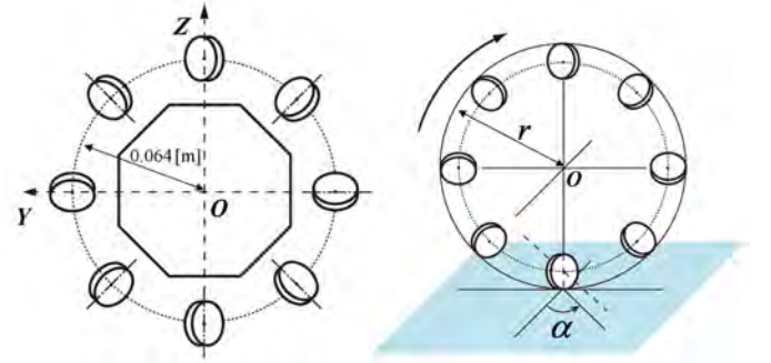
Fig. 8. Simplified screw model (left: front view, right: relation to the ground)
