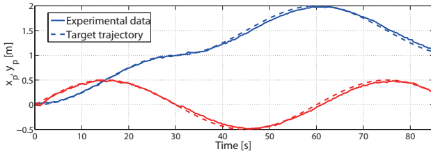
Fig. 21. Time plot of x_p and y_p in experiment (feedback)
