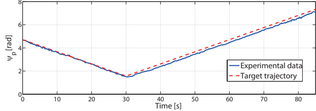
Fig. 22. Time plot of \psi_p in experiment (feedback)
