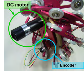
Fig. 2. Screw drive unit
