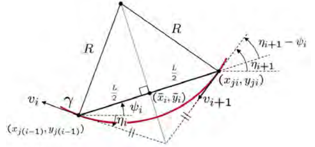
Fig. 18. Target path between two joints
