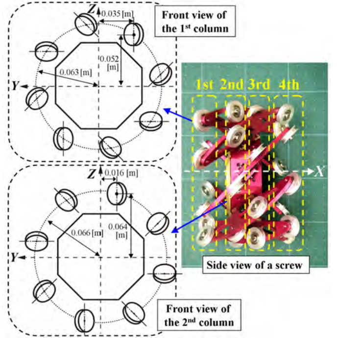
Fig. 7. Side and front views of a screw (left screw drive unit)
