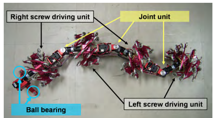
Fig. 1. Snake-like robot using the screw drive mechanism
