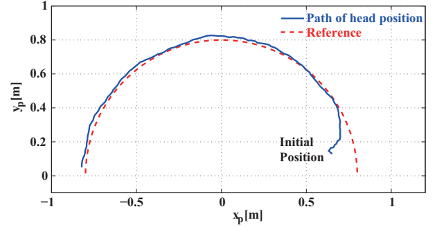
Fig. 15. x - y plot of the head position in experiment (feedback)
