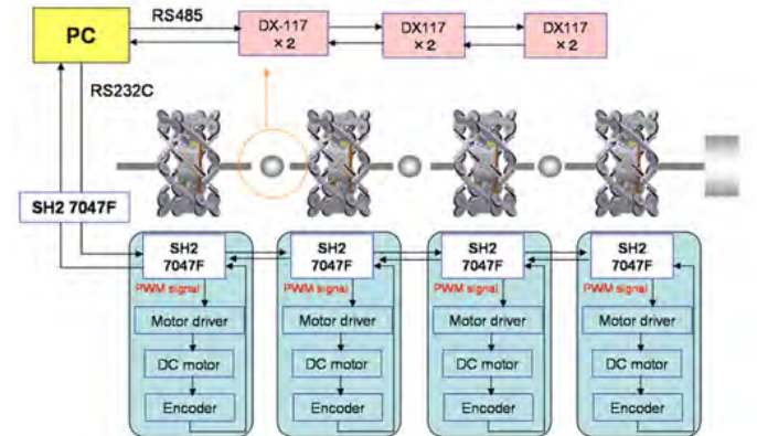
Fig. 4. Schematic of control system
