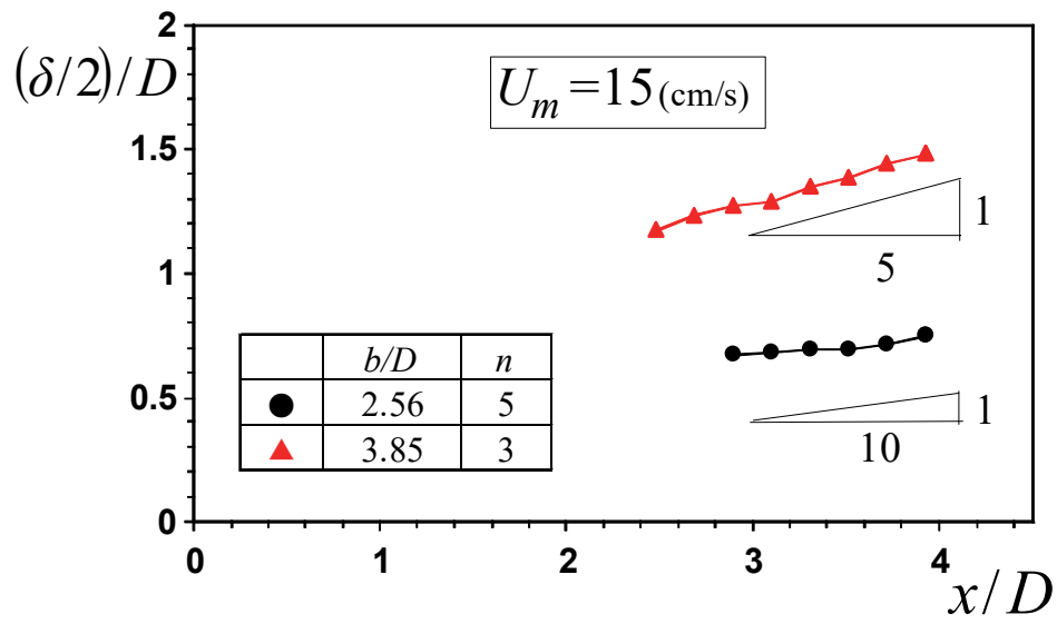
Fig.9 Longitudinal variations of high-speed streak half-width varying the allocation density under the constant bulk-mean velocity U_m = 15 \text{ cm/s} : The high-speed streak width is larger in sparser allocation, irrespective of downstream distance from the cylinder, because original width corresponds with the slit width d defined by cylinders allocation.
