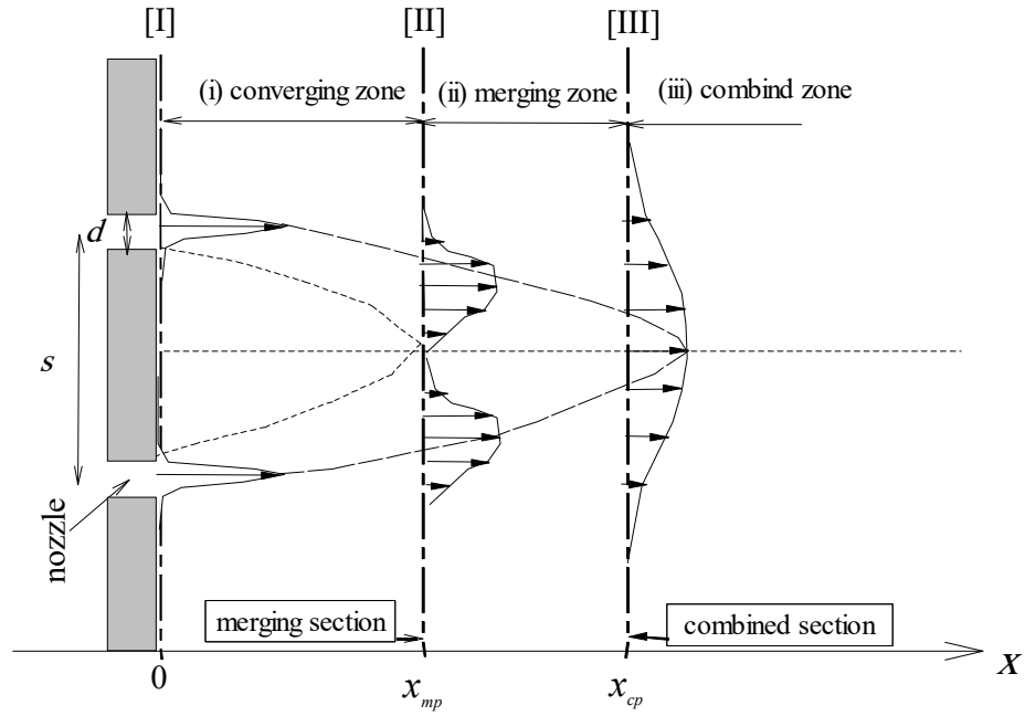
Fig.7 Phenomenological flow models and classification of characteristic zones in the streamwise direction: (a) flow passing one-line cylinders, (b) two parallel jets
