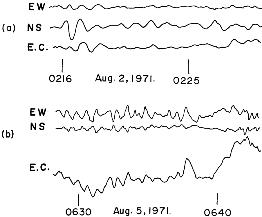
Fig. 4. Examples in which the variation of one component ( (a) north-south and (b) east-west) of geomagnetic fields is dominant. It is seen in (a) that telluric field shown by E. C. does not resemble magnetic field especially from middle to last part of curves, but in (b) the telluric field resembles EW component of magnetic field. The length of a time interval of 10 minutes give sensitivities of each field, and they are 0.43 \gamma/\text{sec} and 0.11 \text{ volt/km} for magnetic and telluric fields, respectively. The senses of the fields are eastward, northward and southward increase towards the top of the paper for magnetic EW, NS and telluric NS components, respectively.
