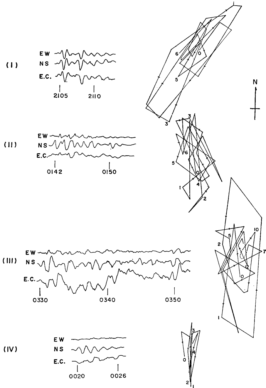
Fig. 2. Four types of hodographs with traces of original curves. Curves are geomagnetic east-west, north-south and telluric north-south components from the top of the paper and their senses are eastward, northward and southward towards the top of the paper. The sensitivities are 0.43 \gamma/\text{sec} and 0.11 \text{ v/km} for geomagnetic and telluric fields, respectively, per variations of the length of time interval of 10 minutes. Events are observed on (i) Aug. 2, (ii) Aug. 2, (iii) Aug. 1 and (iv) Aug. 2. Time marks on the figure do not show accurate time.
