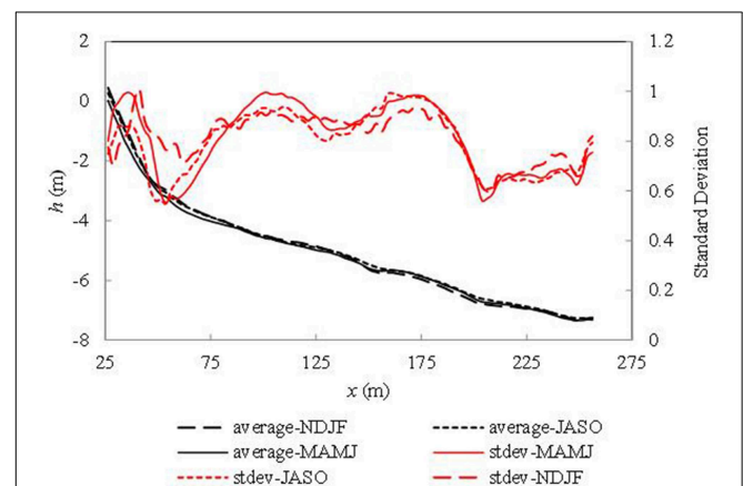
FIGURE 6 | Seasonally averaged beach profiles at J-O Coast. Black lines—seasonally averaged beach profiles, red lines—standard deviation.
