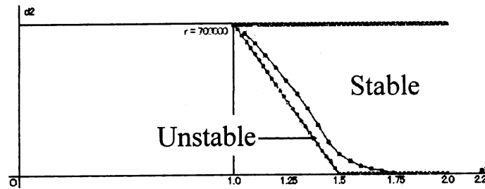
Figure 3.9: Stability and instability
