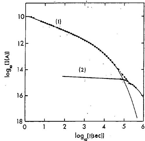
Fig. 4. Discharge current of PVA at 26.85°C. (1) Current calculated by the Kohlrausch function with \beta_k=0.470 , \tau^*=2.53 \times 10^3 s, and \epsilon_0 - \epsilon_\infty = 7.44 . (2) Current calculated by the Debye equation with \tau_m = 4.4 \times 10^5 s, and \epsilon_0 - \epsilon_\infty = 0.51 . The discharge current is proportional to -d\phi(t)/dt .
